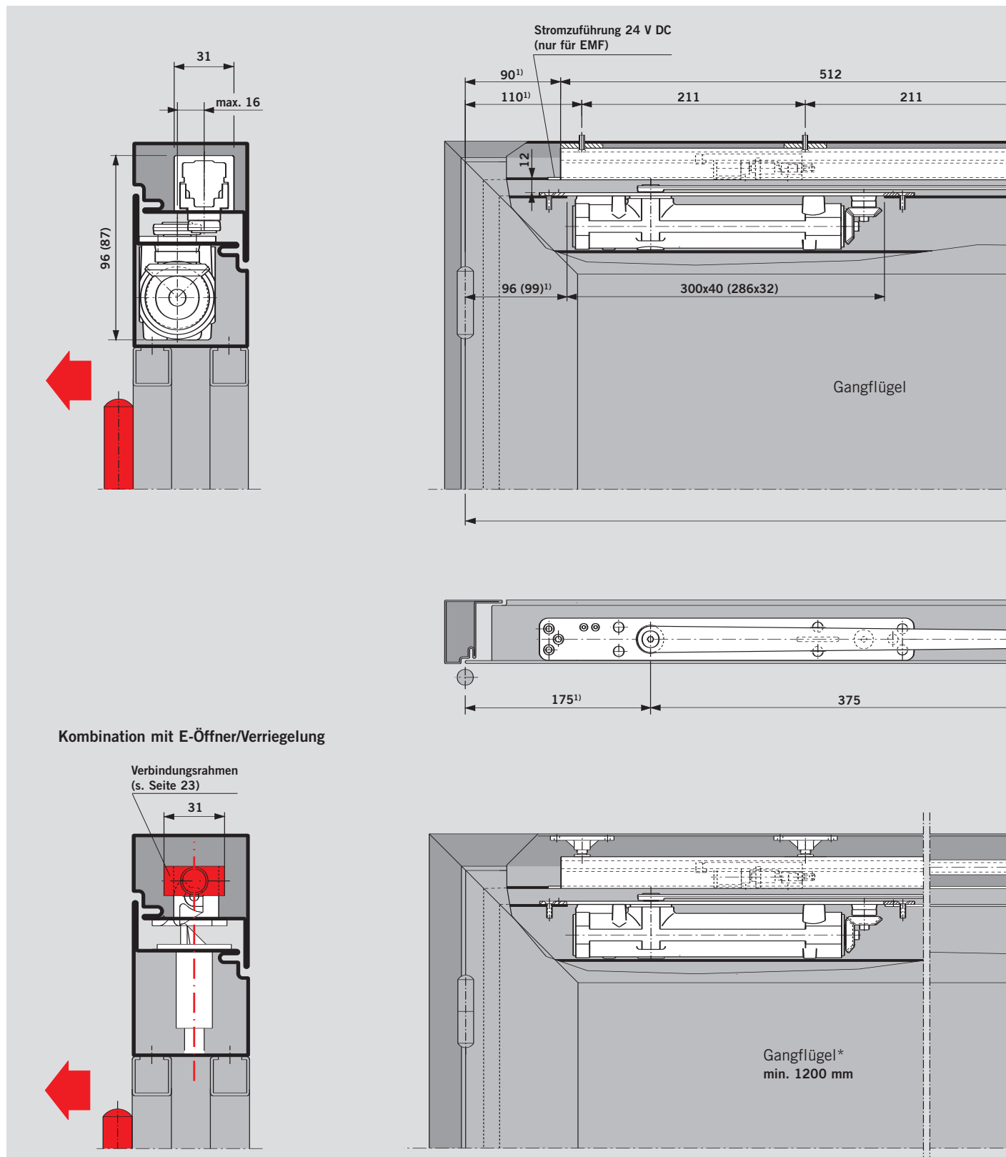
Abbildung ITS 96 3 - 6 ( ) Maße = ITS 96 2 - 4
